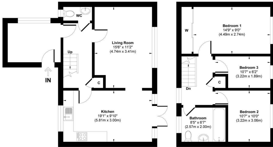
Ground Floor Approximate Floor Area 520 sq.ft (48.27 sq.m)
